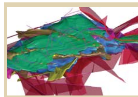
Mineralised bodies and fault system
